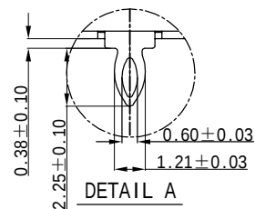
DETAIL A SCALE 4:1 QUANTITY:6
