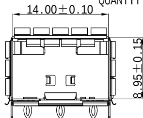
DETAIL B SCALE 4:1 QUANTITY:9
