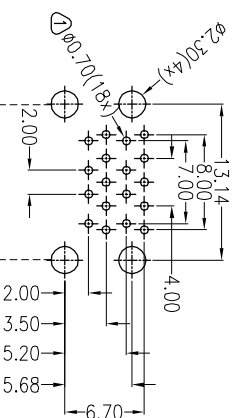
P.C.B LAYOUT (COMPONENT SIDE) DEFAULT TOLERANCE:±0.05
