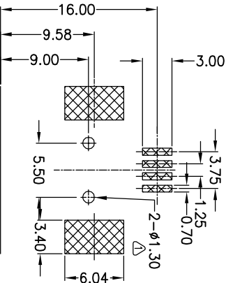
RECOMMENDED P.C.B HOLE LAYOUT TOP VIEW(TOLERANCE±0.10)
