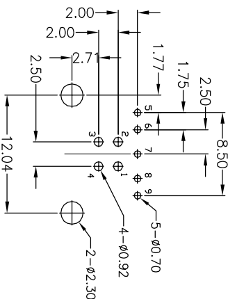
RECOMMENDED P.C.B HOLE LAYOUT TOP VIEW(TOLERANCE:±0.10)
